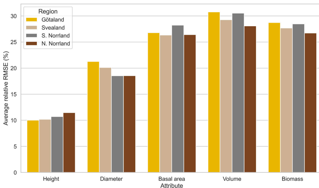
Fig. 9. Region-wise average relative RMSE values across 50 experiments over the forest attribute predictions. The relative RMSE estimates are obtained with the CNN model.
