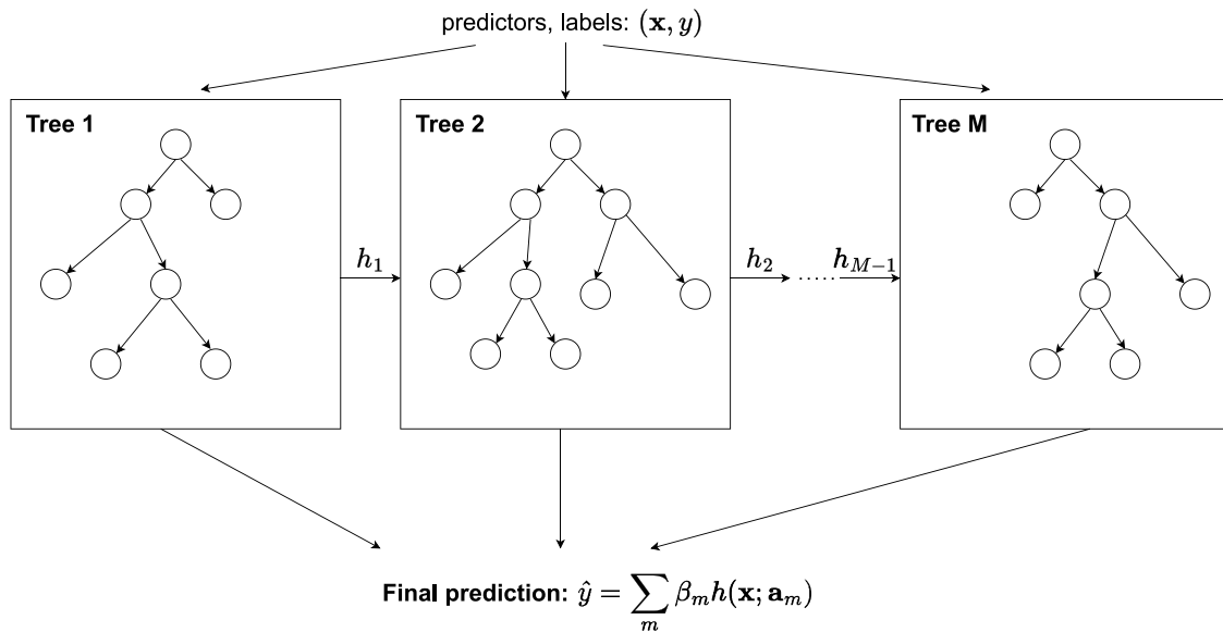
Fig. 4. General scheme for XGBoost. A series of regression trees are fitted on the predictors and corresponding labels. In our case the predictors are represented by 60 ALS metrics along with region, scanner type and leaf-on/leaf-off condition, whereas the labels are measurements from the NFI plots. Each tree's residuals are used for fitting the next tree. The final prediction is an additive expansion of all fitted trees.
