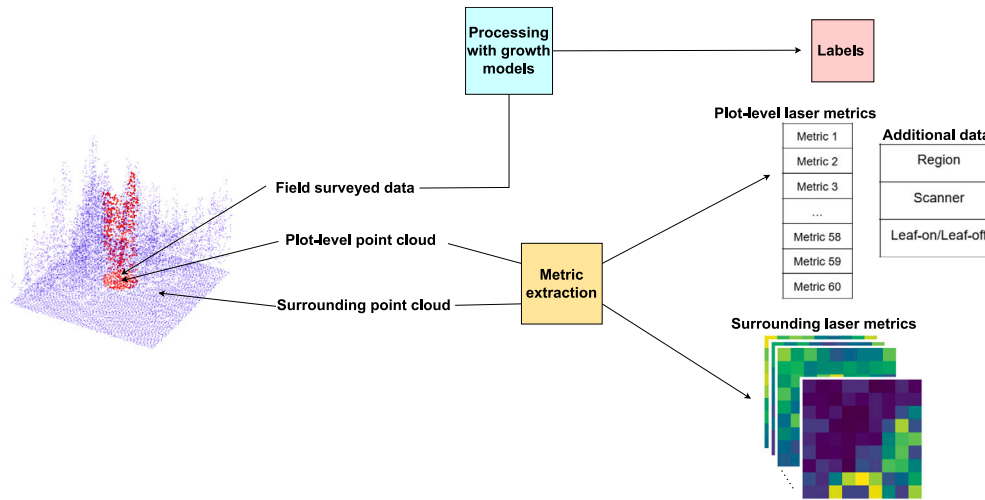
Fig. 1. Data processing. ALS point clouds were collected over 90m×90m areas centered on NFI plots. Plot-level ALS metrics were computed by clipping the point cloud to the extent of each plot, while surrounding-area ALS metrics were calculated across the full 90 m × 90 m area using 10 m × 10 m grid cells. In both cases, 60 ALS metrics were computed. Additional inputs included region, scanner type, and leaf-on/leaf-off condition. The field data (used as labels) were adjusted with allometric growth models to match the date of scanning.
