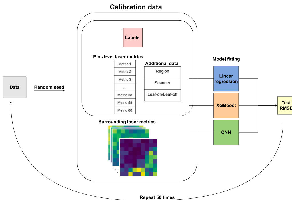
Fig. 6. Evaluation methodology used in the experiments. The dataset was randomly split into a calibration set (95%) and a test set (5%). For the ML approaches, 15% of the calibration set was used for validation. The approaches were evaluated on the test set, and this process was repeated 50 times. The baseline linear regression models and XGBoost used plot-level ALS metrics, whereas the CNN incorporated even surrounding ALS metrics.
