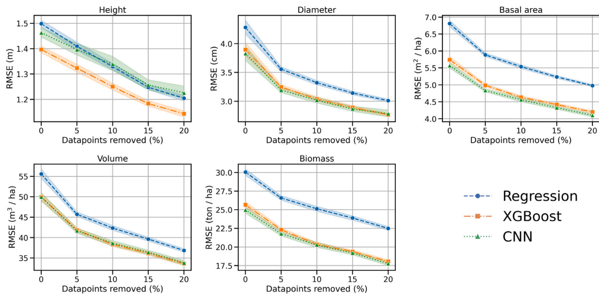
Fig. 10. Average RMSE values with 95% confidence intervals over the five different datasets used in the sensitivity analysis. The results are presented for all of Sweden.
